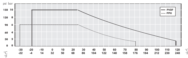
DN65 - DN100 (PPH, PVDF, ABS)
